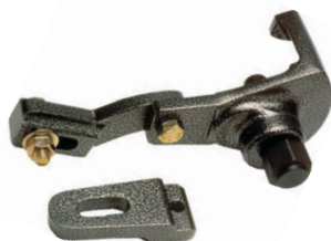
Multi-Adjustable Slack Adjuster Puller for Haldex units. Accommodates left offset, right offset and standard elongated arm designs from either side. TGT-10410
