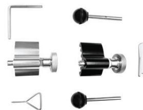
VW and Audi Timing Tool Kit For VAG 2.0L TDI PO DOHC engines on A4, A6, Jetta, Golf, etc. CTA-2777
